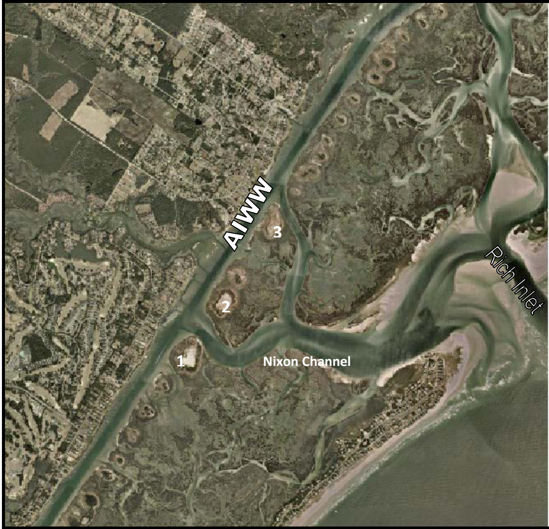
Figure 3.8. Location of AIWW dredged material disposal sites 1, 2, and 3.
