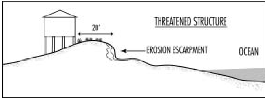
Figure 2.8. Diagram depicting imminently threatened structures (NCDCM, 2003a)
