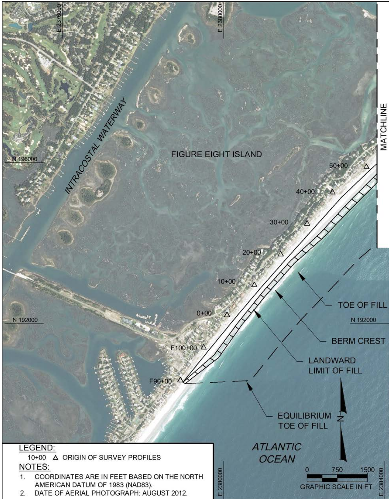
Figure 3.6b. Alternative 4: Southern portion of beach fill; 2012 shoreline conditions.
