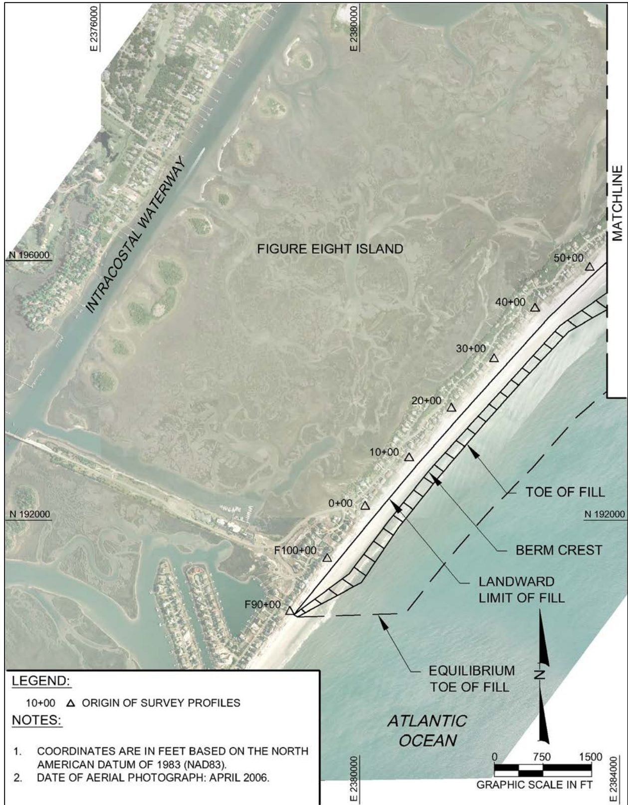
Figure 3.4d. Alternative 3: Southern portion of beach fill; 2006 shoreline conditions.
