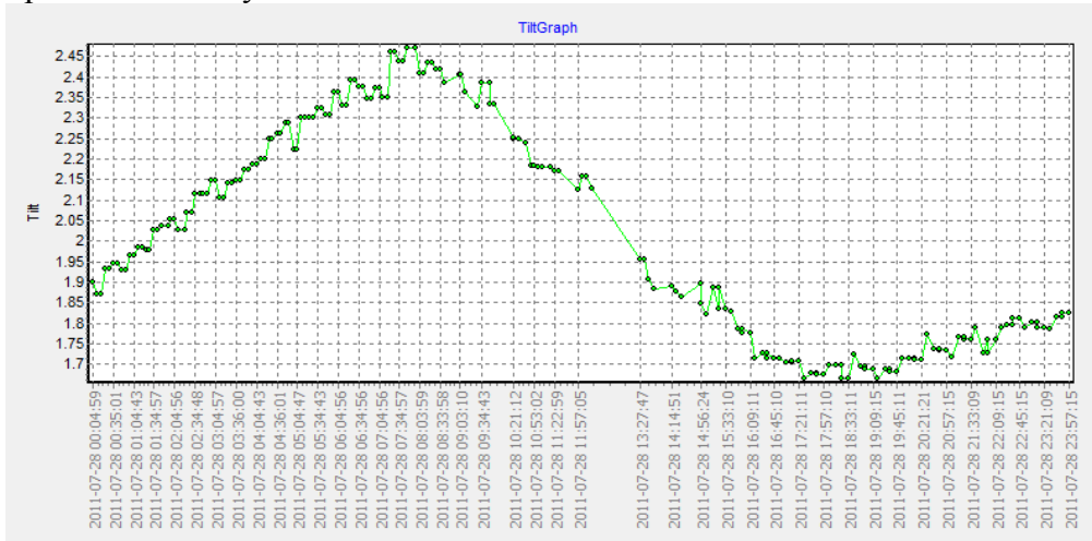
Figure 9: Bearings tilt variation during 24-hour period
