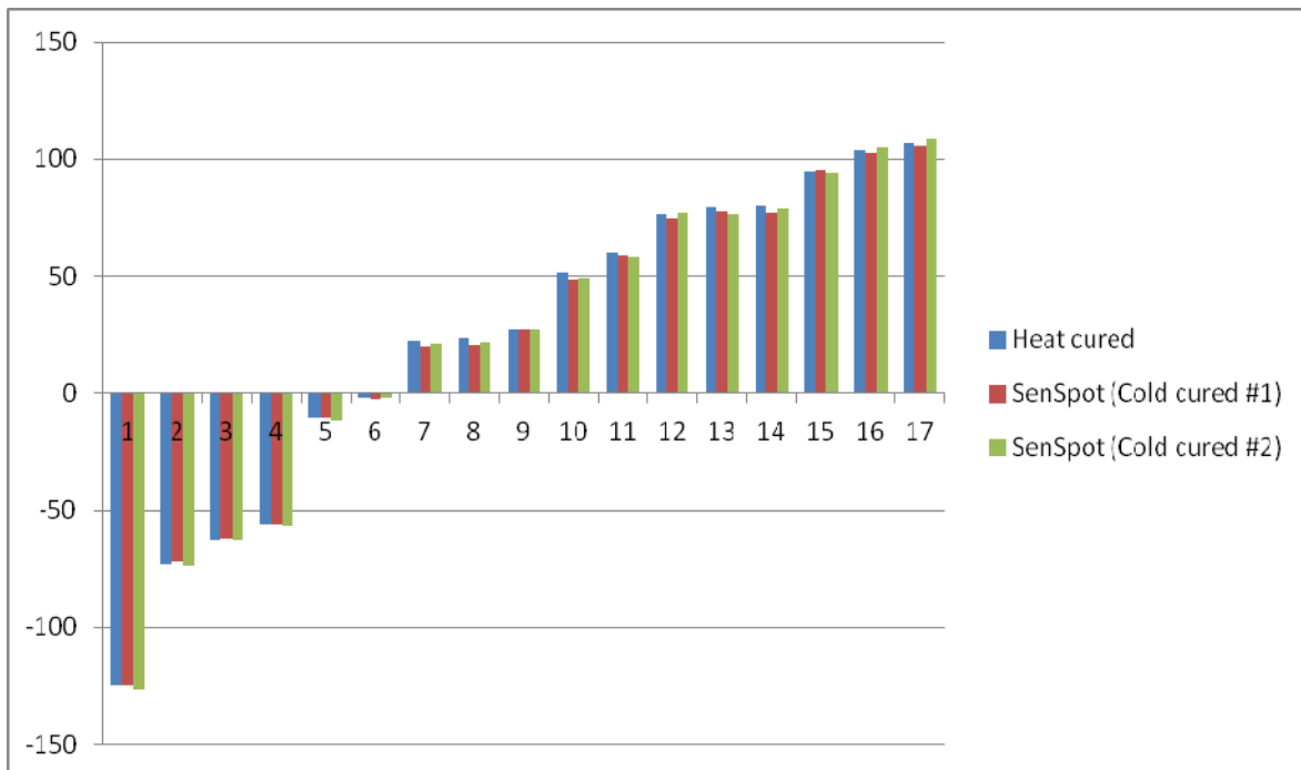
Figure 7: The comparison of the strain readouts of the heat cured system and two SenSpot sensors with cold cured strain gauge attachment.
