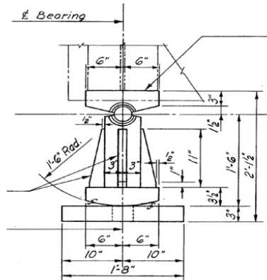
Figure 10: The schematic of rocker bearings, per design sheets of the bridge.
